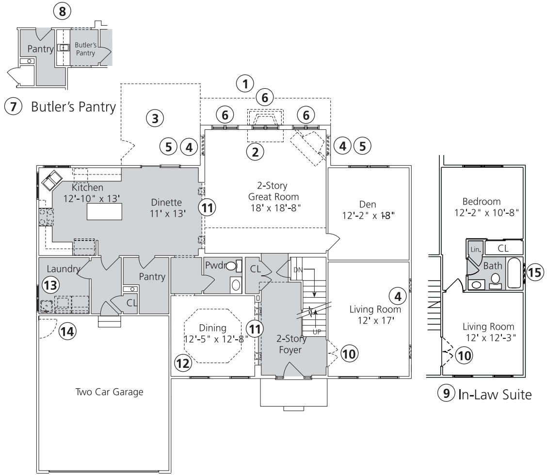
First Floor (Elevation "A")
