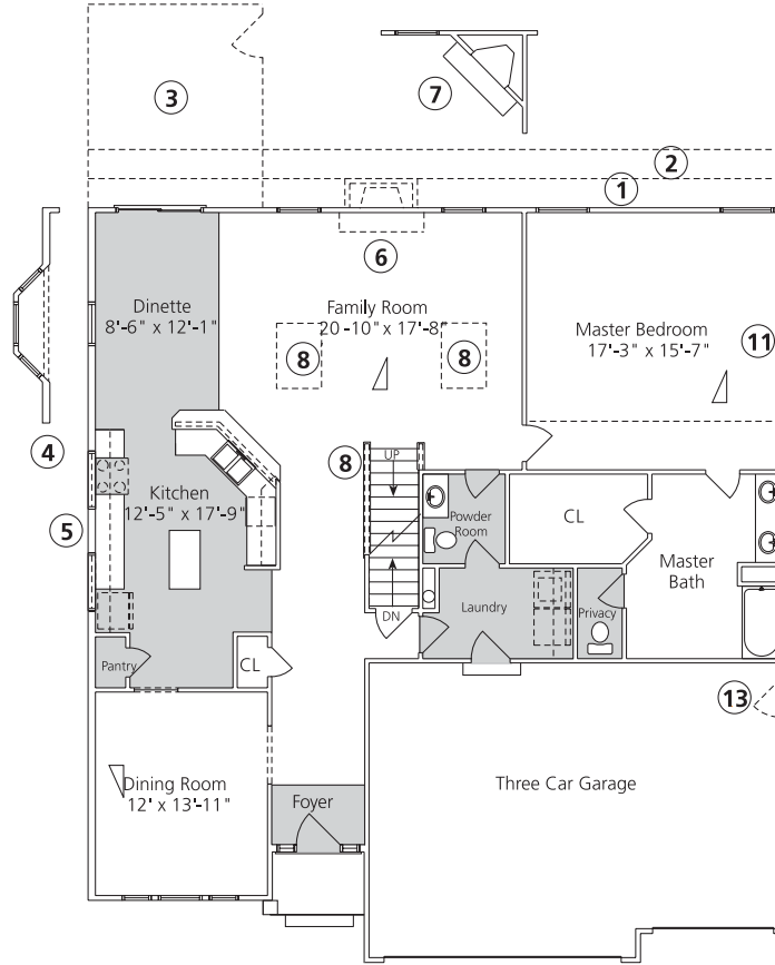
First Floor (Elevation "A")
