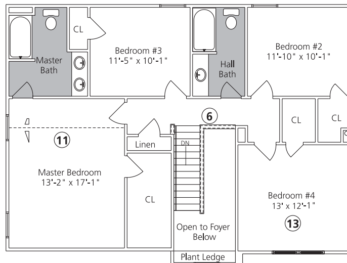
Second Floor Plan (Elevation "A")
