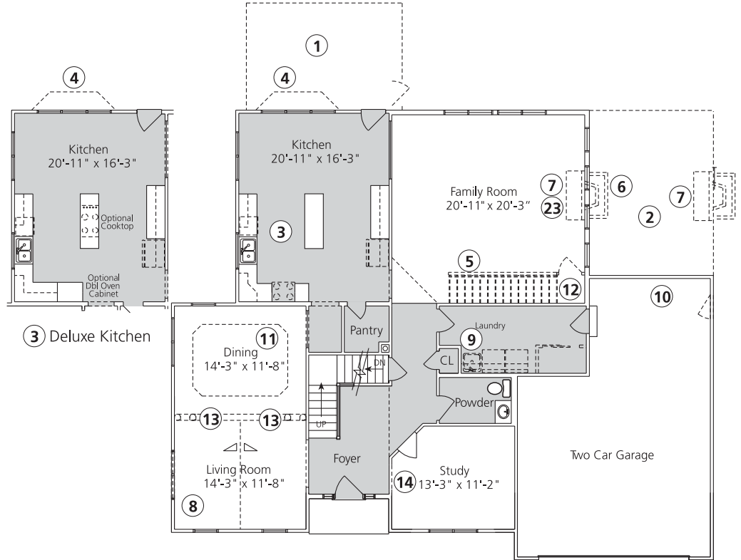
First Floor (Elevation "A")
