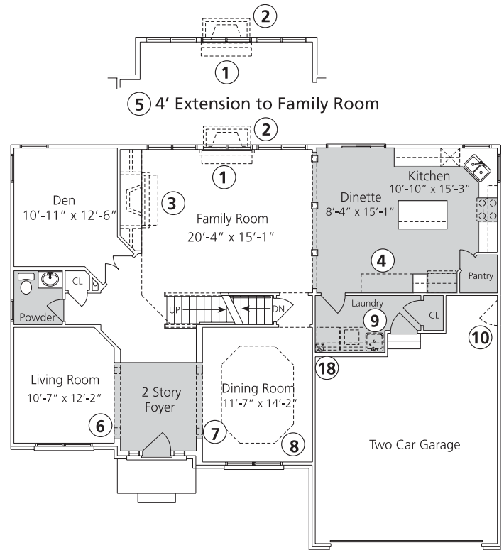
First Floor (Elevation "A")
